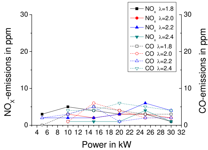
Figure 10 NO x - and CO-emissions for different powers and excess air ratios
