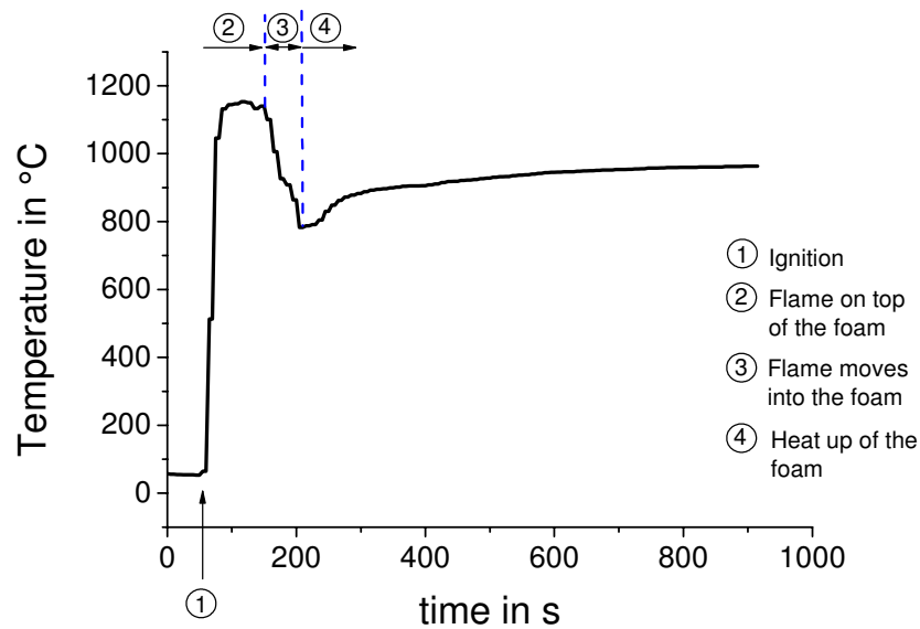
Figure 8 Temperature development during start up
