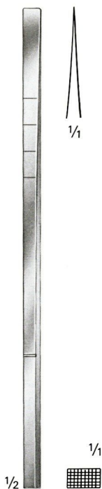
Cottle 56.363-04 4 mm 56.363-06 6 mm 56.363-07 7 mm 56.363-09 9 mm 56.363-12 12 mm 18 cm/7"
